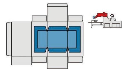
Window with pre-heated creasing lengthwise and shaped die cut
